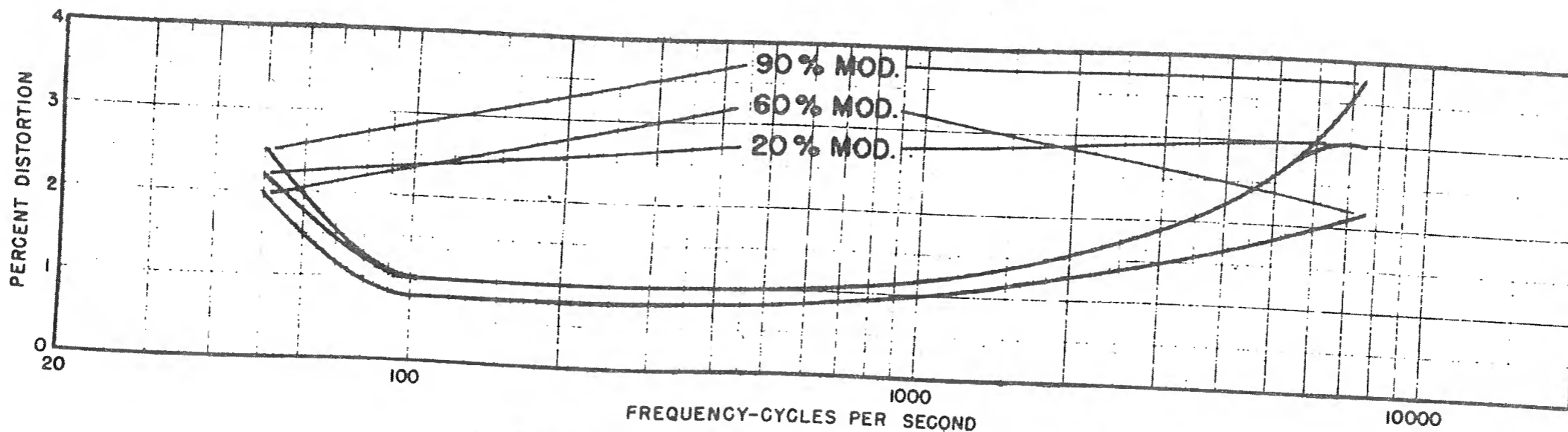
AUDIO FREQUENCY HARMONIC DISTORTION
